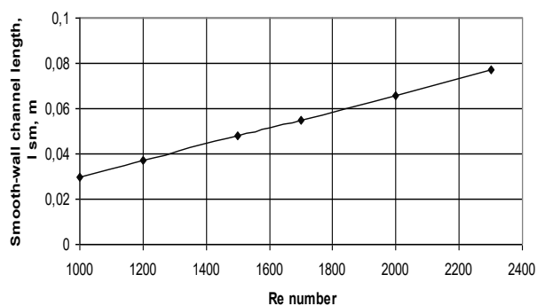
Figure 5 - Length of a smooth-wall steam generating channel l_{sm} , m ( T_s=360^\circ\text{C} )
