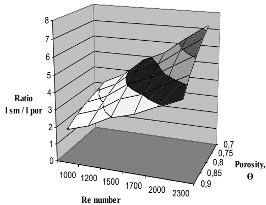
Figure 1 - The value of geometric coefficient of the porous steam-generating channel efficiency k_F=l_{\text{sm}}/l_{\text{por}} ( T_s=360^{\circ}\text{C} )
