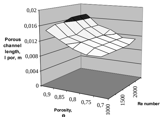
Figure 6 - Length of porous steam generating channel l_{por} , m ( T_s=360^\circ\text{C} )
