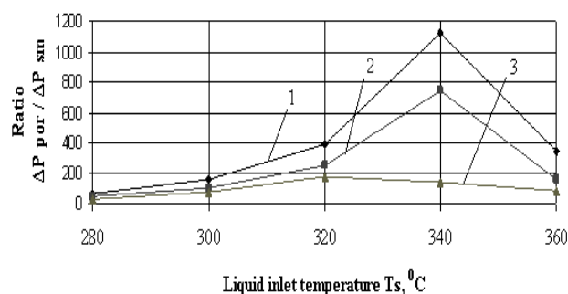
Figure 8 - Dependence \Delta P_{por} / \Delta P_{sm} = f(T_s) for different Reynolds numbers of the flow at the channel inlet
